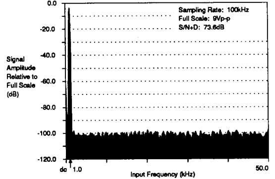
Figure 19. Plot of CS5012A with 1 kHz Full Scale Input
