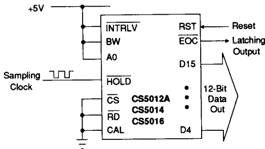
Figure 8. Microprocessor-Independent Connections
