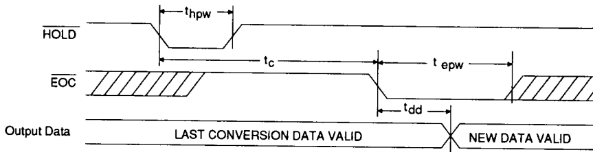
Conversion Timing
