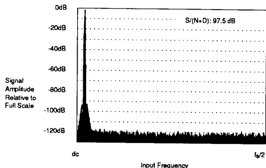
Figure 23. Plot of Ideal 16-bit ADC
