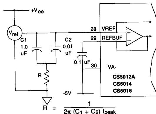
Figure 10. Reference Connections
