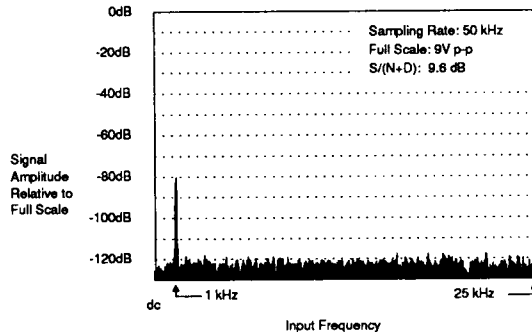
Figure 29. CS5016 FFT plot with 1 kHz -80 dB Input
